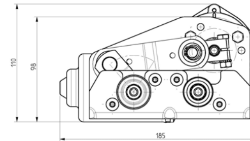
COMPLETE WIPER MECHANISM (LINKAGE + DC GEARMOTOR Ø62-35)
