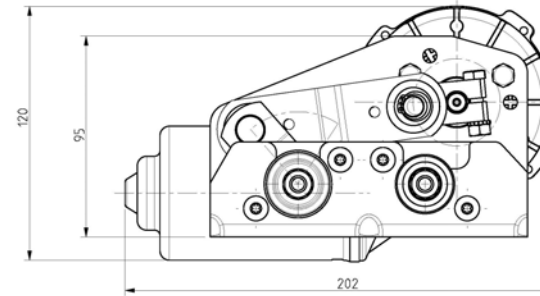
COMPLETE WIPER MECHANISM (LINKAGE + DC GEARMOTOR Ø62-43)
